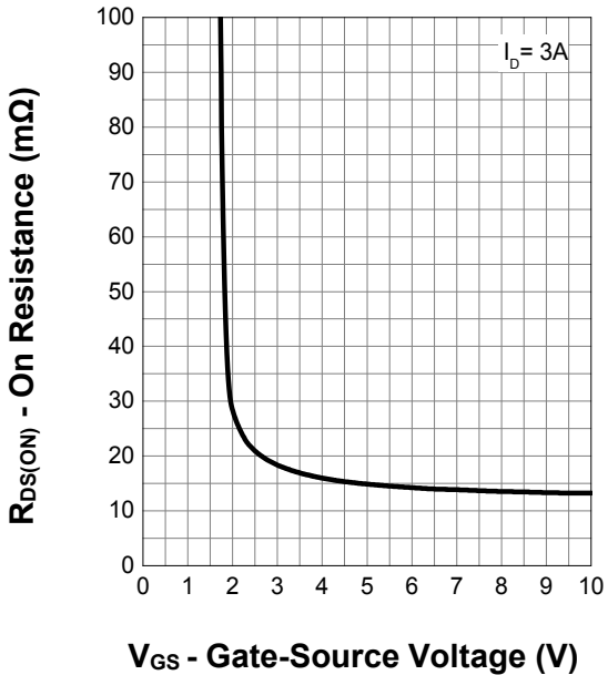
Transfer Characteristics
