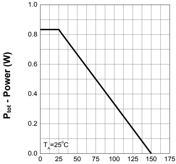
Power Capability
