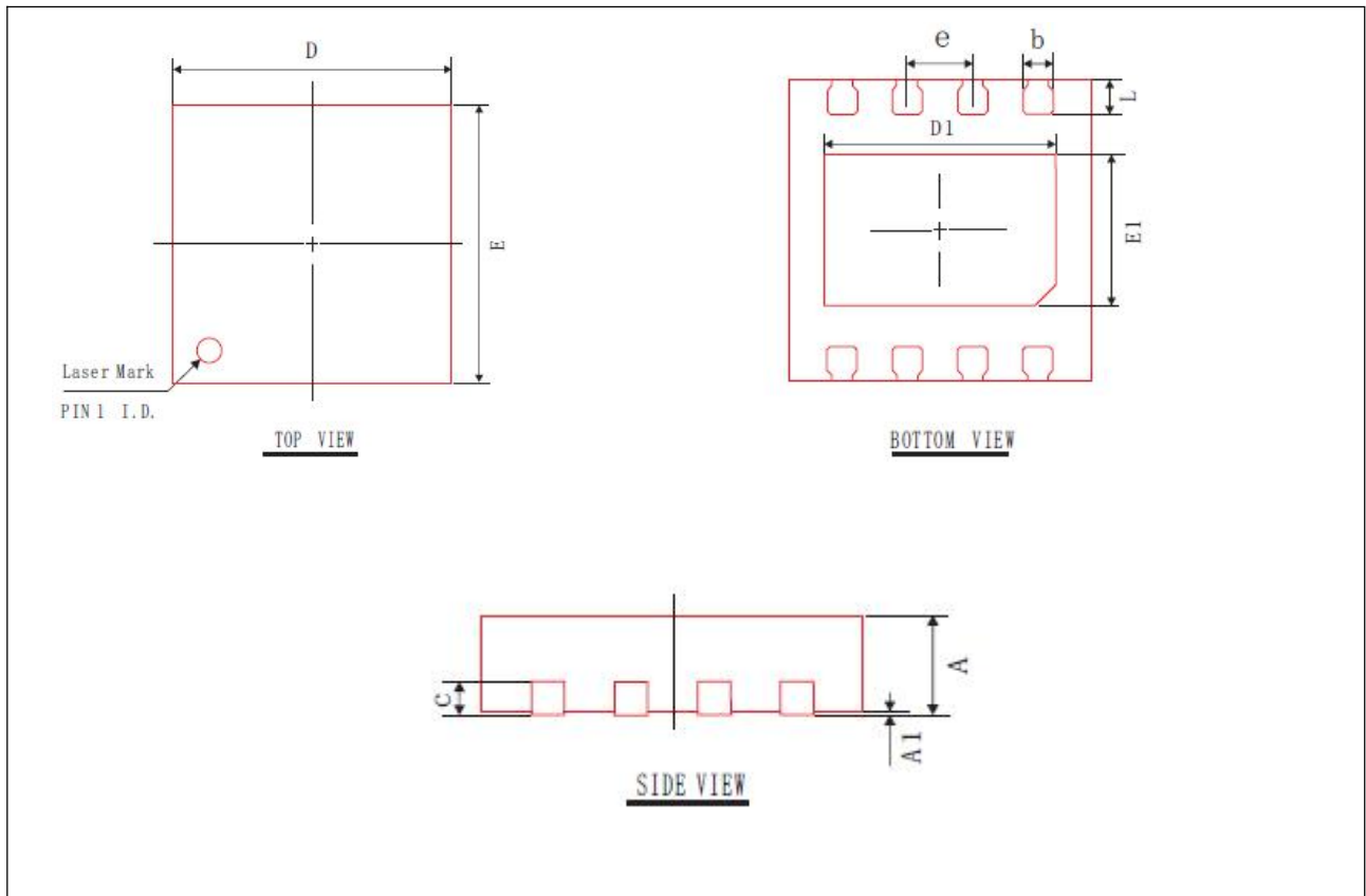
DFN3x3 - 8L Package
